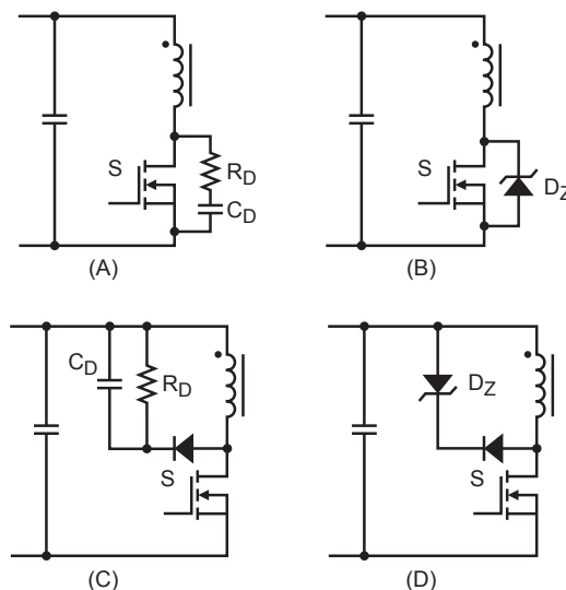
Figure 5—Snubber Designs
