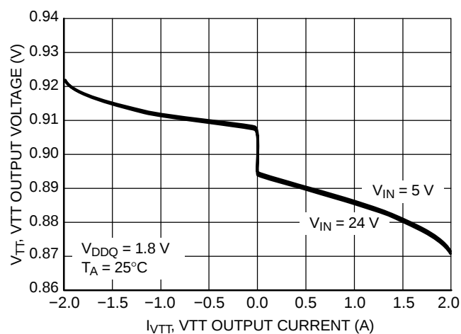
Figure 12. VTT Output Voltage (DDR2) vs. VTT Output Current
