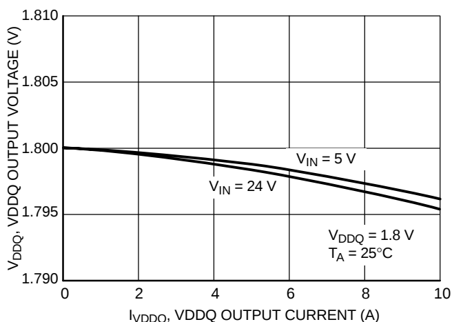
Figure 10. VDDQ Output Voltage vs. VDDQ Output Current
