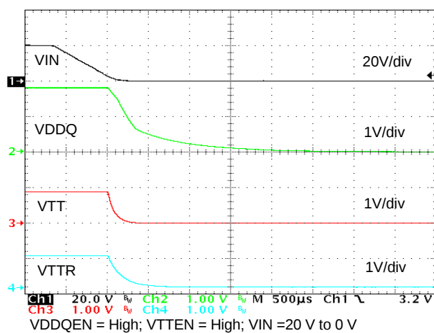
Figure 18. Power-Down Waveforms
