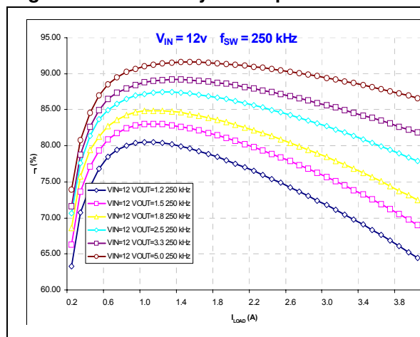
Figure 35. Efficiency vs. output current
