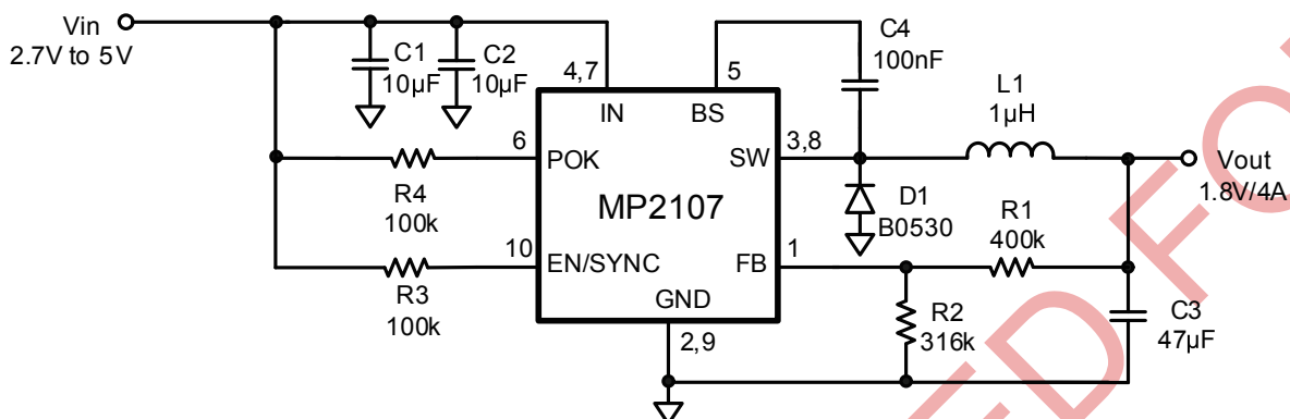
Figure 4—Typical application circuit of MP2107
