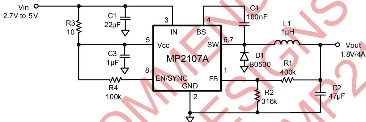
Figure 5—Typical application circuit of MP2107A
