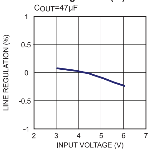
Line Regulation (%)
