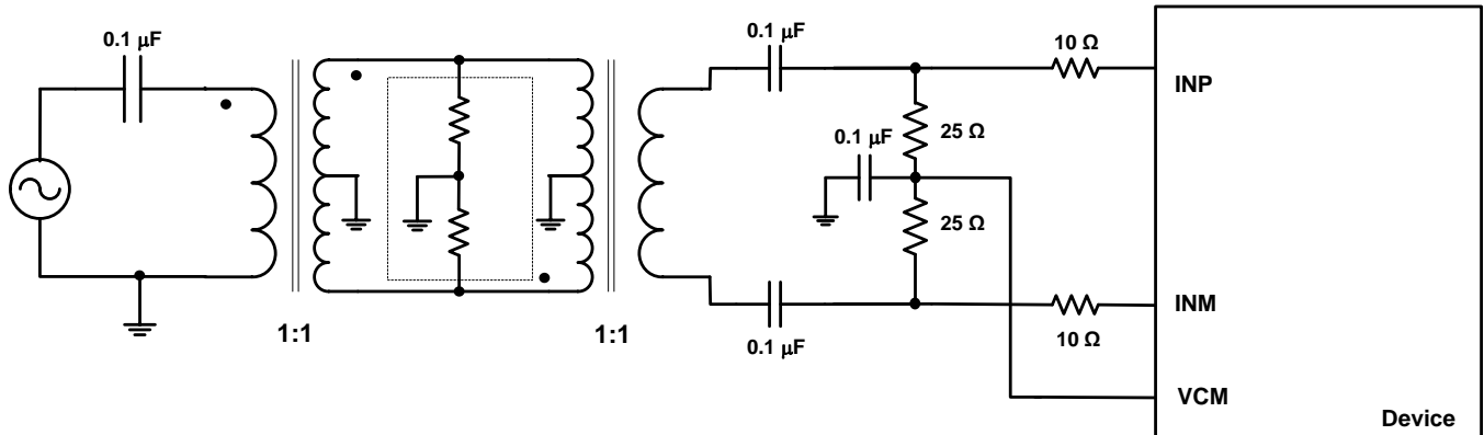
Figure 178. Driving Circuit for High Input Frequencies ( f_{IN} > 230 MHz)
