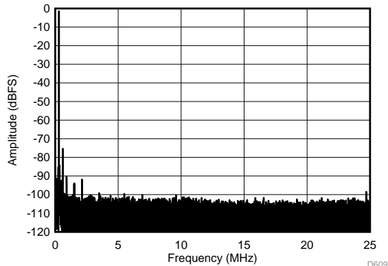
SFDR = 68.2 dBc, SNR = 67.4 dBFS, SINAD = 67.3 dBFS, THD = 86.4 dBc, HD2 = 68.2 dBc, HD3 = 87.3 dBc
