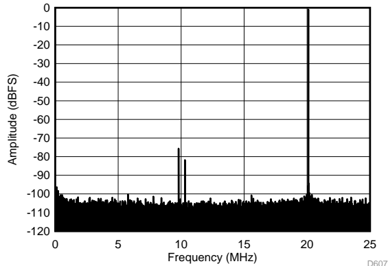
SFDR = 74.7 dBc, SFDR = 95.2 dBc (non 23), SNR = 69.2 dBFS, SINAD = 68.1 dBFS, THD = 73.7 dBc, HD2 = 74.7 dBc, HD3 = 80.9 dBc
