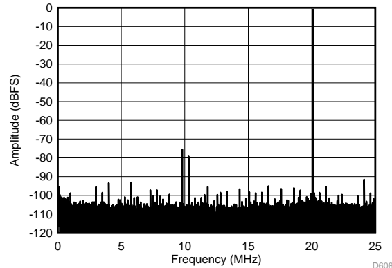
SFDR = 74.5 dBc, SFDR = 91.1 dBc (non 23), SNR = 69.4 dBFS, SINAD = 68.1 dBFS, THD = 72.9 dBc, HD2 = 74.5 dBc, HD3 = 78.2 dBc
