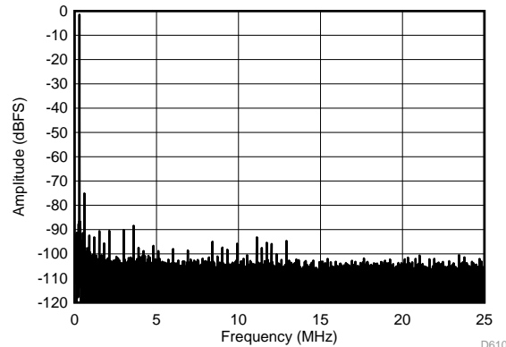
SFDR = 68.1 dBc, SNR = 67.7 dBFS, SINAD = 67.6 dBFS, THD = 86.6 dBc, HD2 = 68.1 dBc, HD3 = 87.3 dBc
