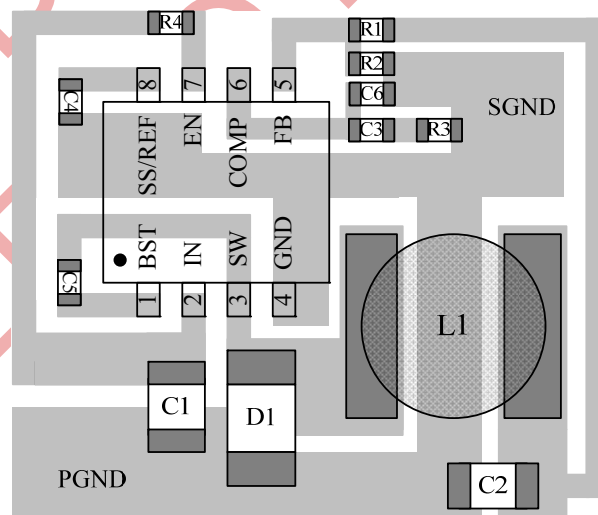
Figure2—PCB Layout
