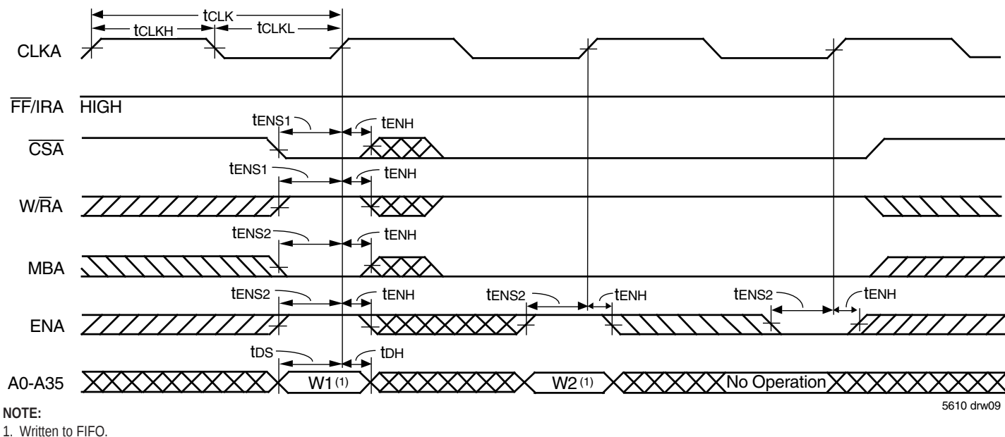
Figure 7. Port A Write Cycle Timing for FIFO (IDT Standard and FWFT Modes)
