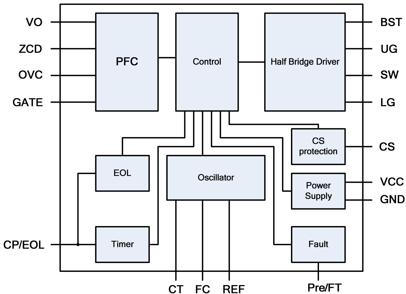
Figure 2— Block Diagram
